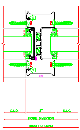
601 I.G. / O.G. H.D. VERTICAL SERIES: 403X - 2" X 4 1/2" SCREWSPLINE
