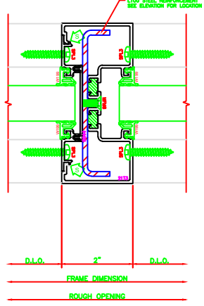
600 I.G. / O.G. VERTICAL SERIES: 403X - 2" X 4 1/2" SCREWSPLINE
